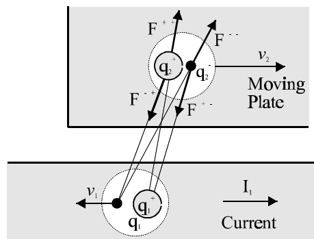
Figure 5. Force between moving charges in an atomic "cell" of two conductors.
