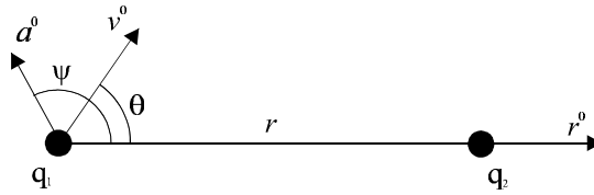
Figure 1. Geometry of electrostatics between charges.
