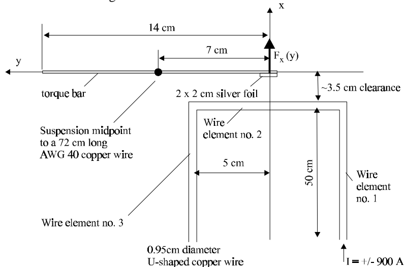
Figure 8. Geometry of the SANSBURY experiment.
